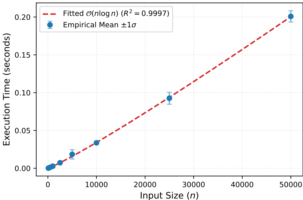
2D Closest Pair D&C: Empirical vs. \mathcal{O}(n \log n) Fit
