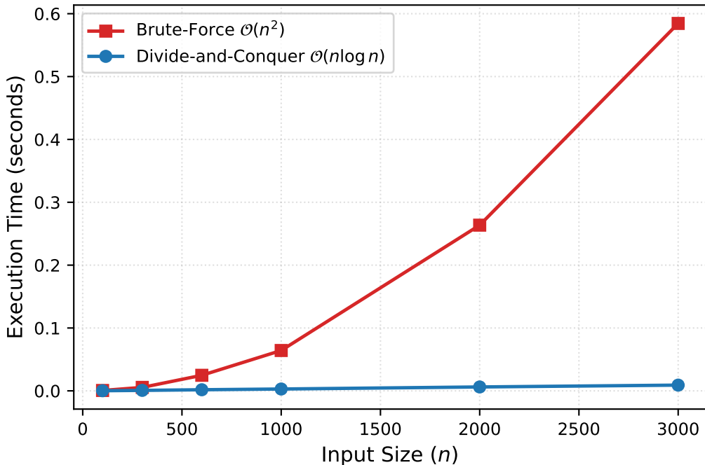
Runtime Comparison: D&C vs. Brute-Force Baseline
