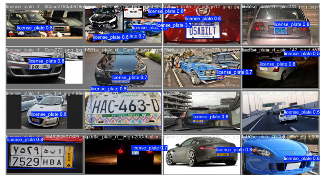
Figure 4: Plate detector ( plate_v1 , GPU server) validation batch predictions. Boxes tightly localise License Plate regions across diverse lighting and angles, confirming mAP50=0.936 on 150-epoch GPU training.
