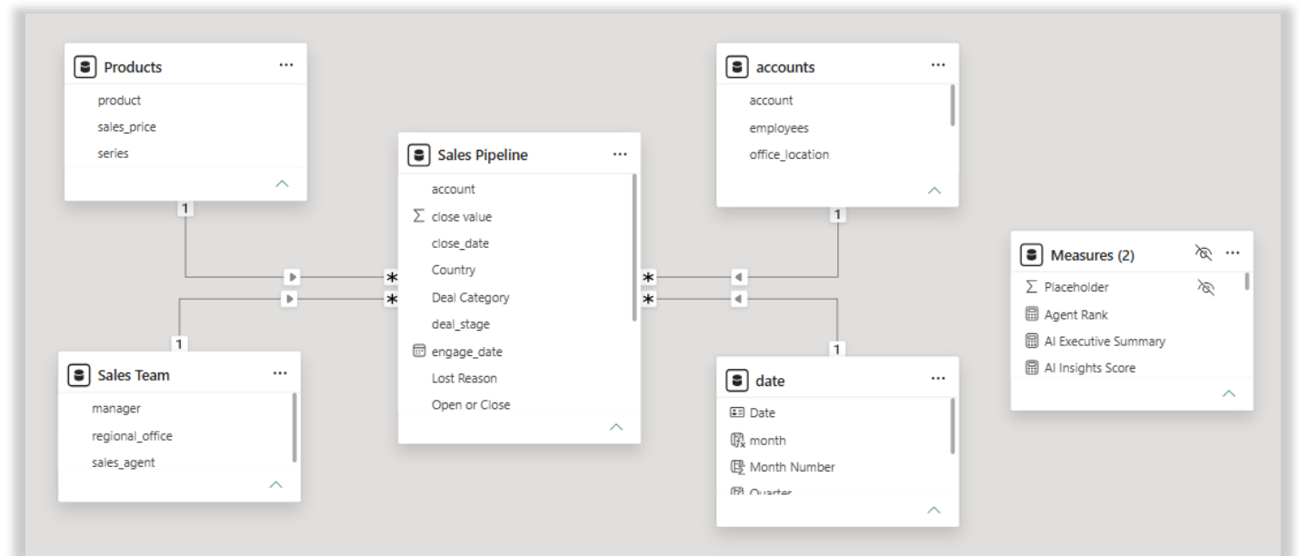
Figure 1: Enterprise Star Schema used for scalable and high-performance Power BI reporting
