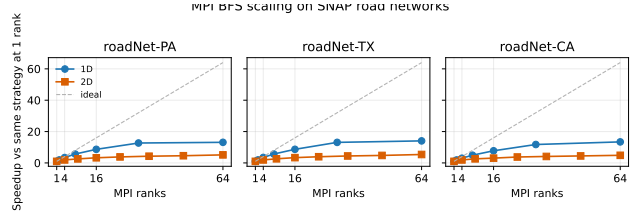
Figure 3: MPI speedup on SNAP road networks. 1D partitioning scales better than the current 2D prototype on these sparse high-diameter road graphs.
