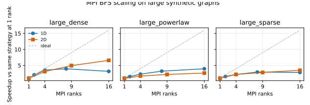
Figure 2: MPI speedup on the large synthetic graphs. Speedup is normalized against the same strategy at one rank.
