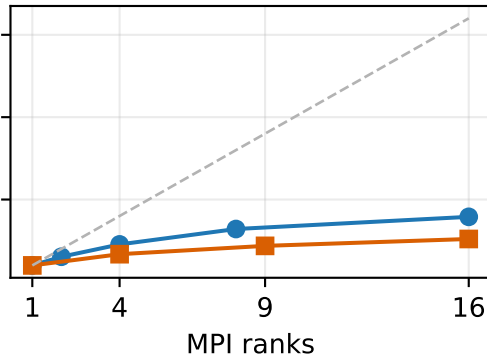
large_powerlaw
