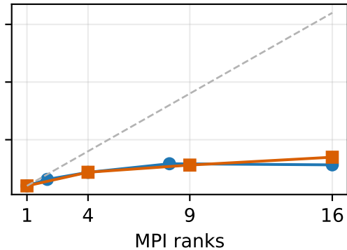
large_sparse
