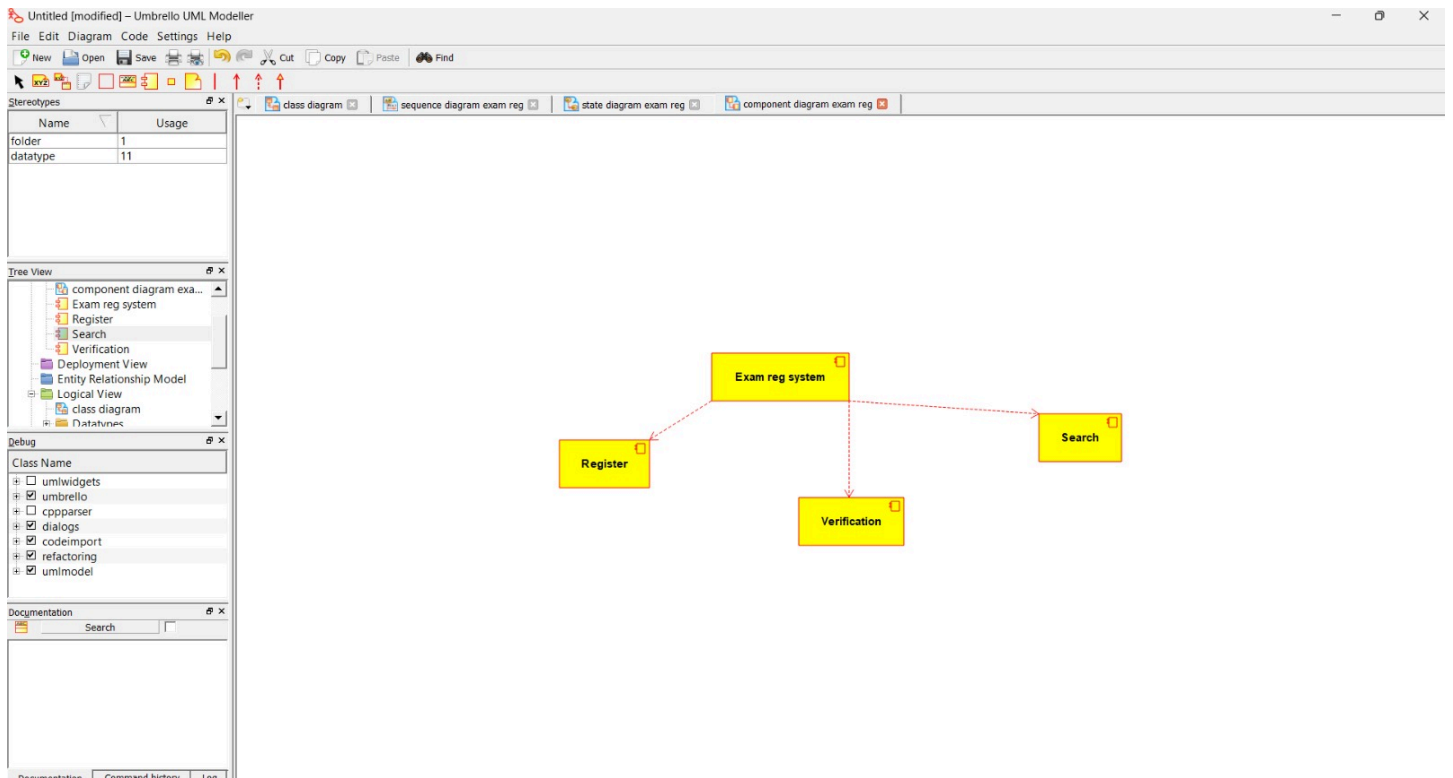
COMPONENT DIAGRAM
