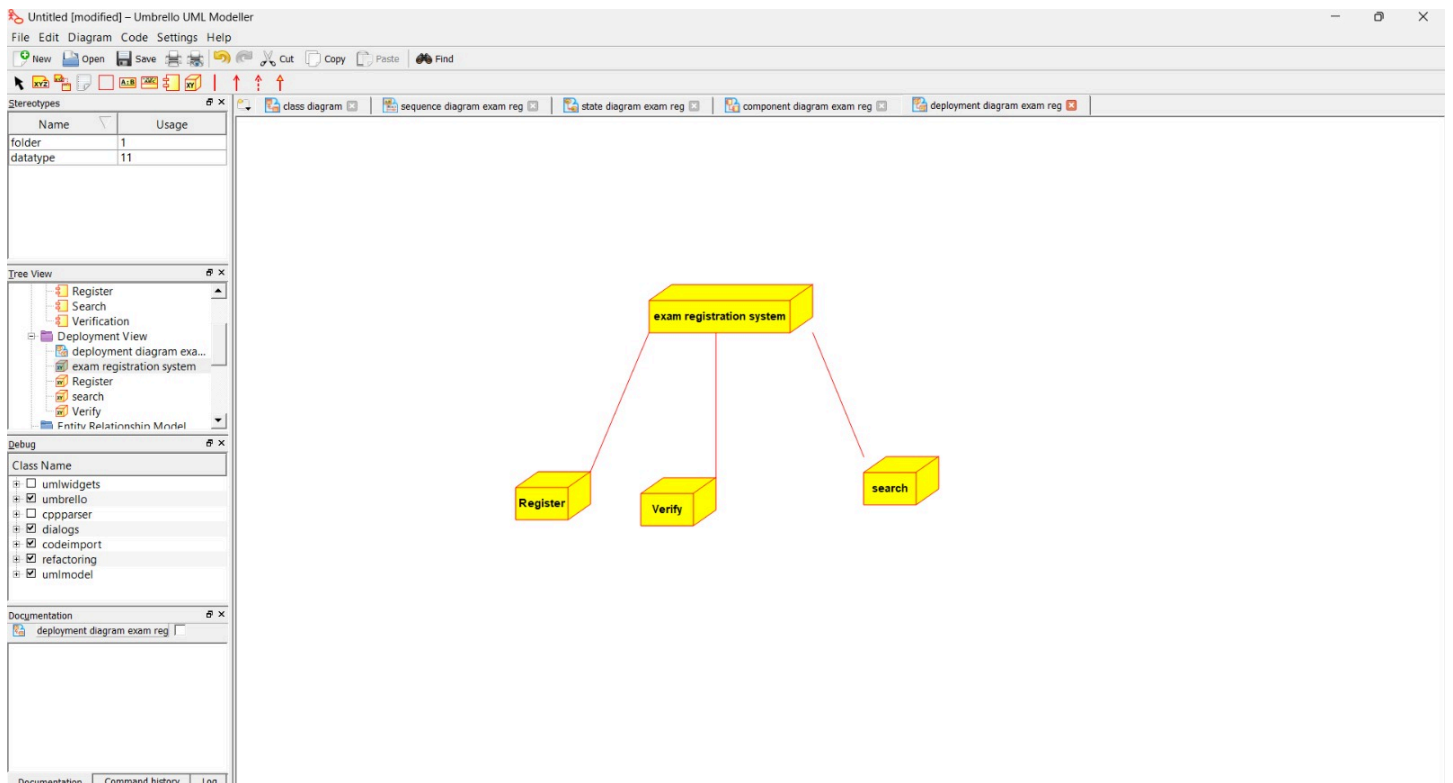
DEPLOYMENT DIAGRAM
