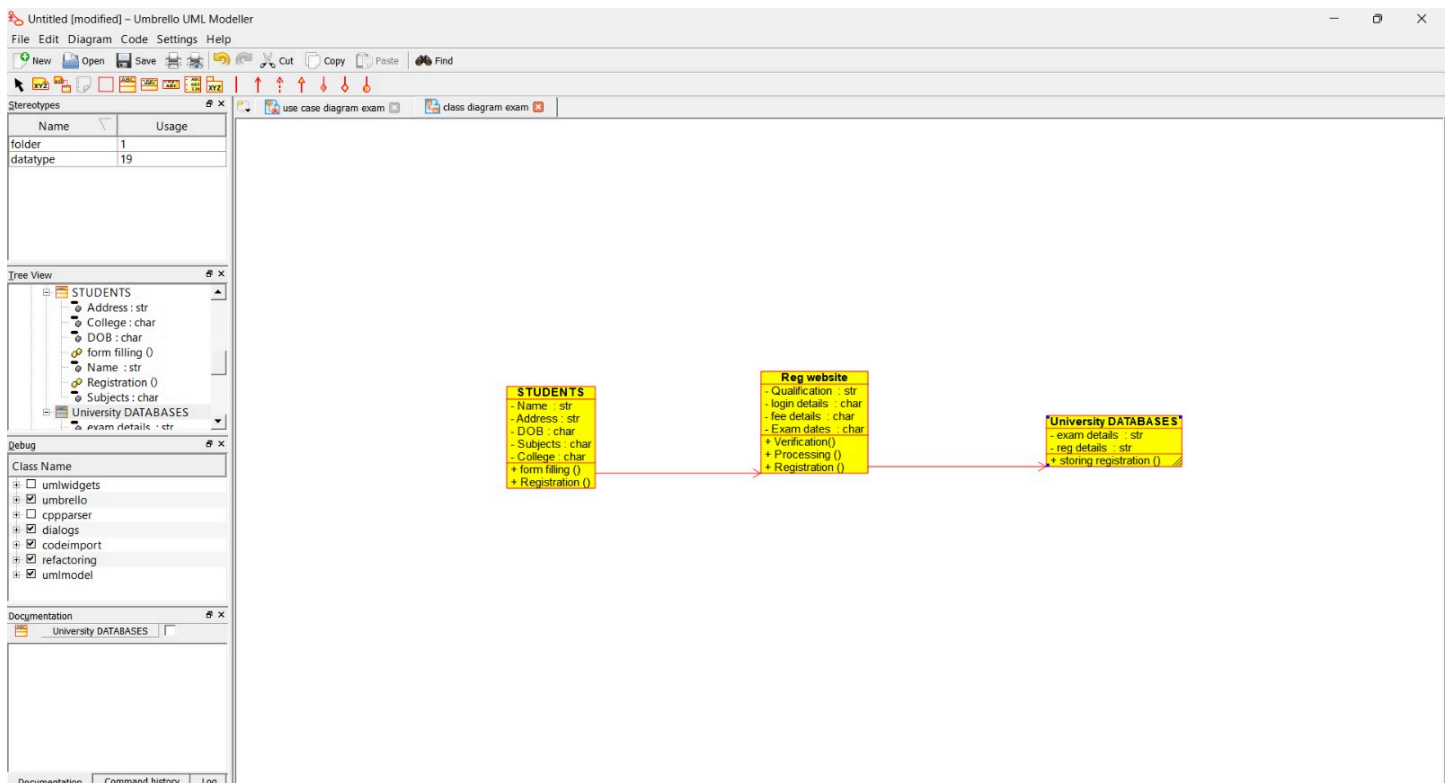
CLASS Diagram
