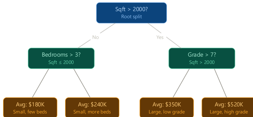
Decision Tree Regressor — Splits leading to average predictions
