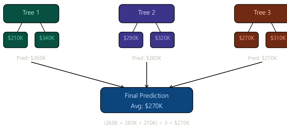
Random Forest — Averaging multiple tree predictions
