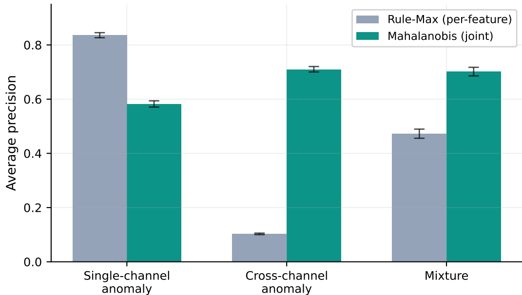
Rules win the obvious case, joint detection wins the subtle one
