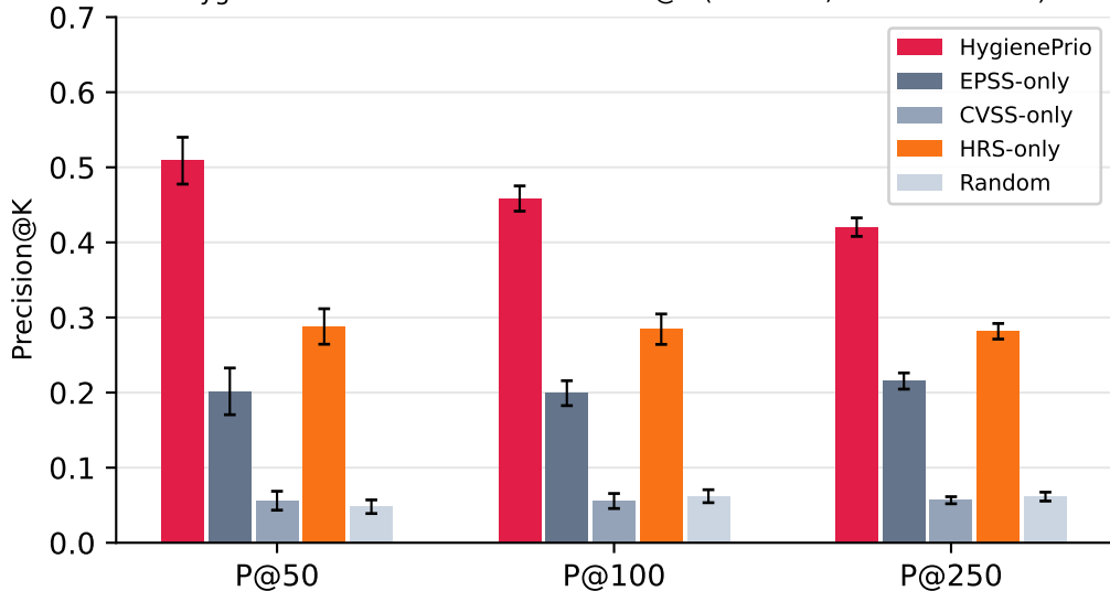
HygienePrio vs. baselines — Precision@K (25 seeds, mean \pm 95% CI)
