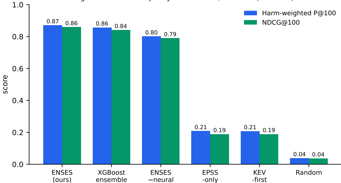
Fig. 2. Prioritization quality on real EPSS/KEV data (25 seeds).
