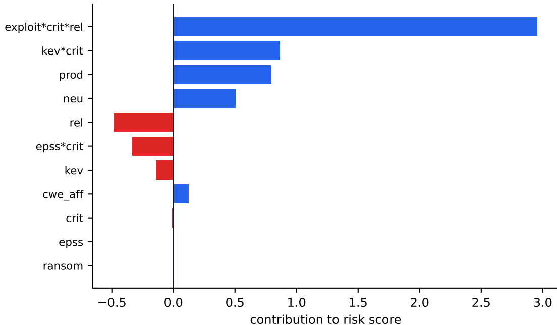
Fig. 4. Glass-box explanation for the top-ranked decision (CVE-2021-22555 on a tier-4 edge compute gateway asset)
