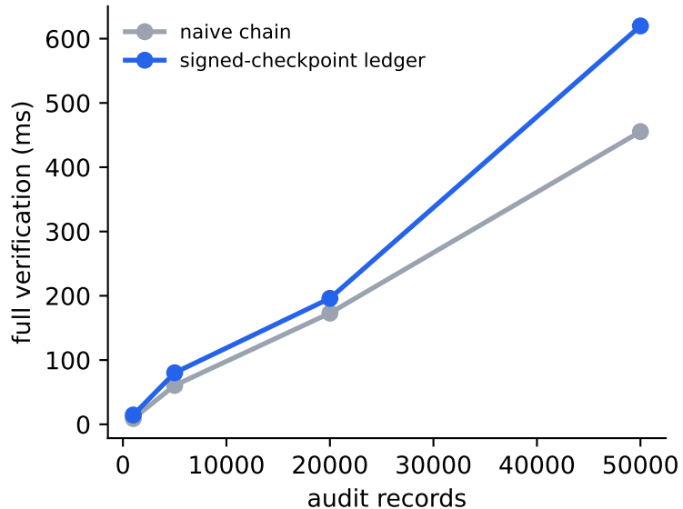
Verification scales linearly
