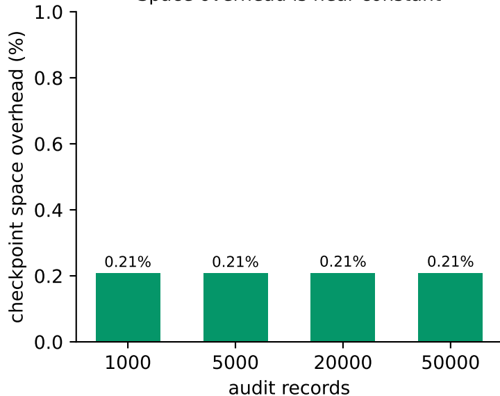
Space overhead is near-constant
