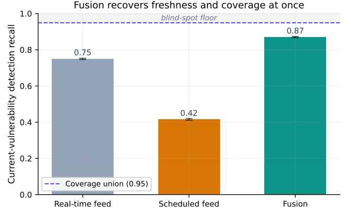
Fig. 1. Detection recall by regime at the reference overlap. Fusion (0.8702) approaches the coverage union, well above the real-time feed (0.7498) and the scheduled feed; the blind spot is the floor that fusion cannot cross.
