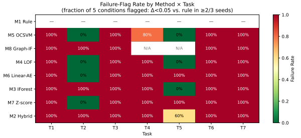
Figure 1: Failure-flag rate heatmap (method \times task). Red cells indicate flagged configurations—ML fails to improve on the rule baseline by the pre-registered \Delta=0.05 threshold (Eq. (1)) in \geq 2/3 seeds; white cells (M8, T4–T5) are not applicable.
