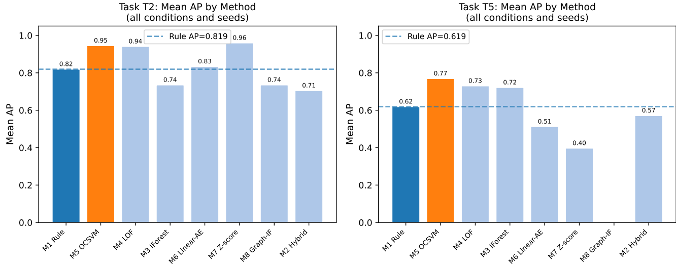
Figure 3: AP by method for T2 (group membership drift) and T5 (patch-vulnerability hygiene), averaged over all conditions and seeds—the two tasks where ML consistently adds value over the rule baseline.
