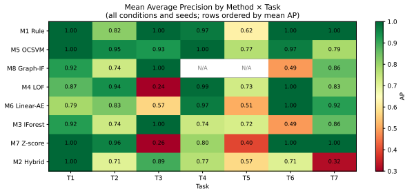
Figure 2: Condition-averaged AP heatmap (method \times task). Higher values indicate better anomaly ranking. Rows are ordered by mean AP across all runs; M1 (rule baseline) anchors the top row.
