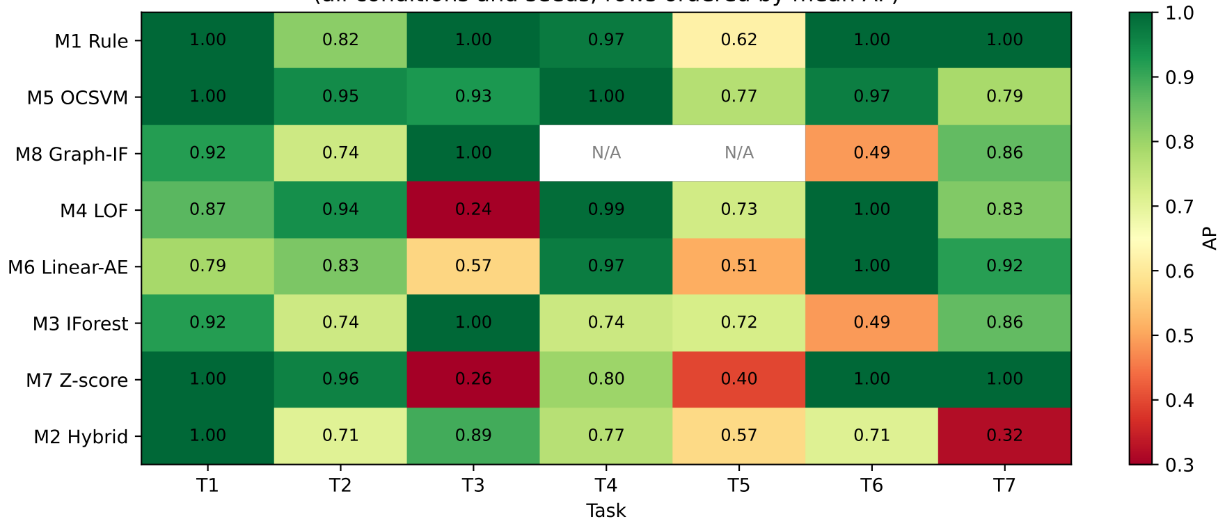
Mean Average Precision by Method × Task (all conditions and seeds; rows ordered by mean AP)
