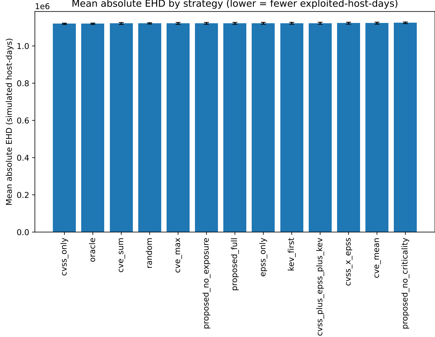
Mean absolute EHD by strategy (lower = fewer exploited-host-days)
