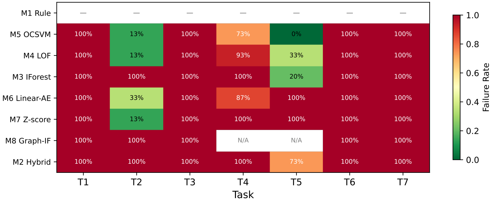
Failure-Flag Rate by Method × Task (fraction of conditions where ML does not beat rule by \Delta=0.05 )
