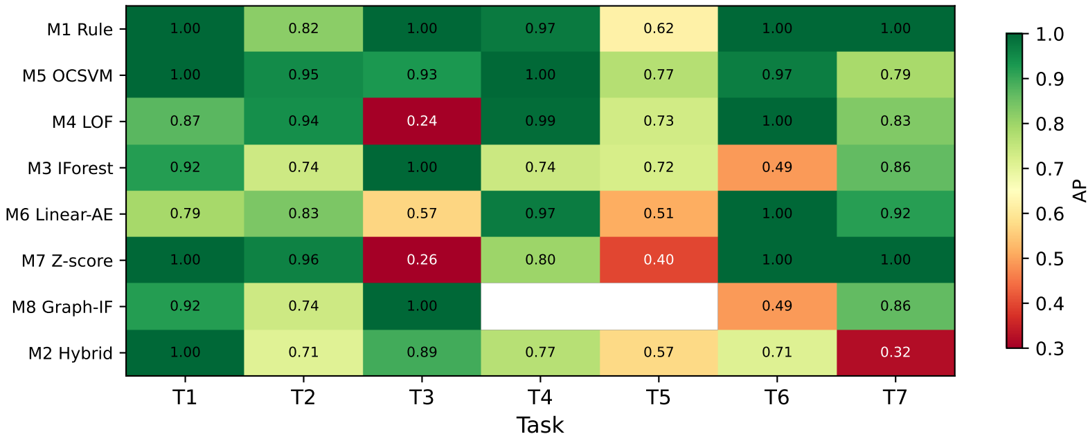
Mean Average Precision by Method × Task (all conditions and seeds)
