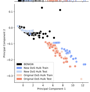
Figure 4: Overlap between train/test sets on CIC 17 via standard evaluation pipeline (Original) vs. our bespoke data (New). Note that the train/test sets of CIC 17 overlap almost entirely.
