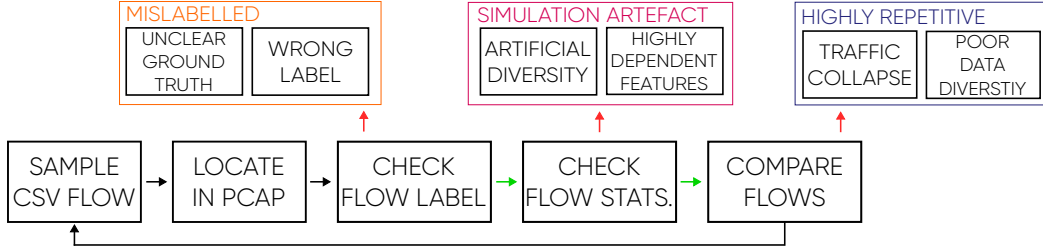
Figure 1: Overview of Manual Analysis Process. To facilitate easier discussion, note that we group our bad smells into three categories: Mislabelled , Simulation Artefact and Highly Repetitive .
