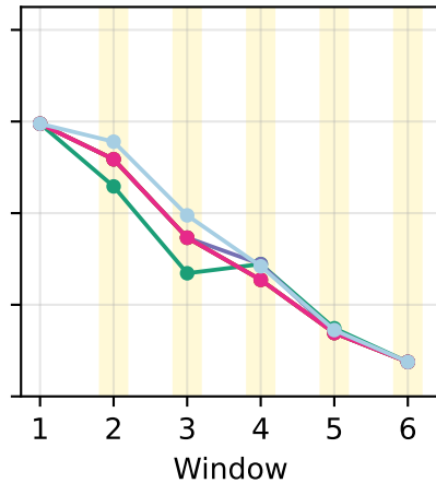
K = 200 ( \tau_K = 0.02 )
