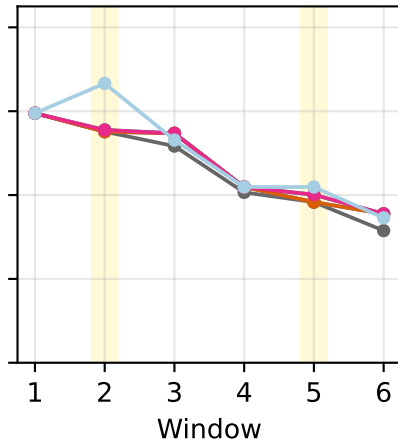
K = 100 ( \tau_K = 0.05 )
