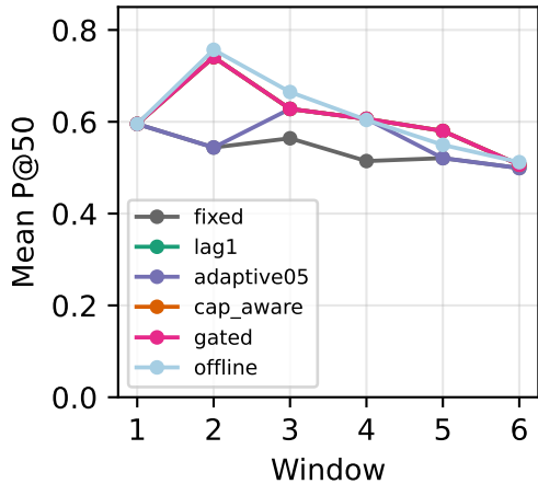
K = 50 ( \tau_K = 0.2 )
