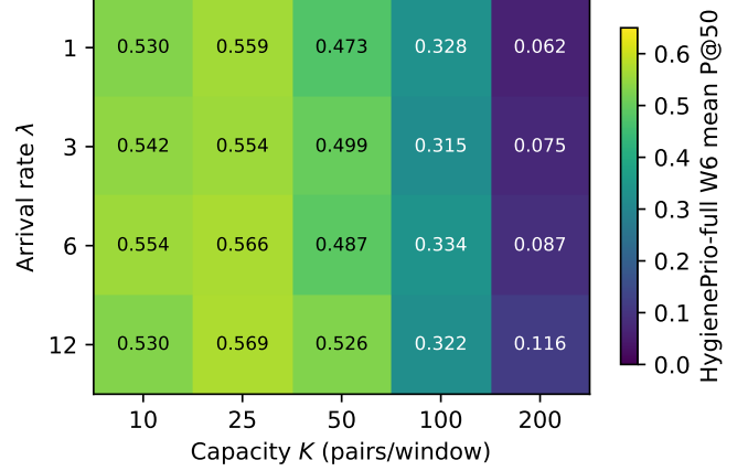
HygienePrio-full W6 retention across (K, \lambda)
