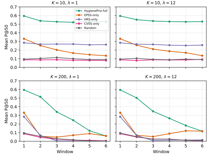
Fig. 3. Mean P@50 trajectories at the four corner cells of the (K, \lambda) grid. At K = 10 (top row), HygienePrio-full holds near 0.55 across windows while EPSS-only decays toward \sim 0.14 . At K = 200 (bottom row), HygienePrio-full also collapses, decaying to \sim 0.06 - 0.12 .
