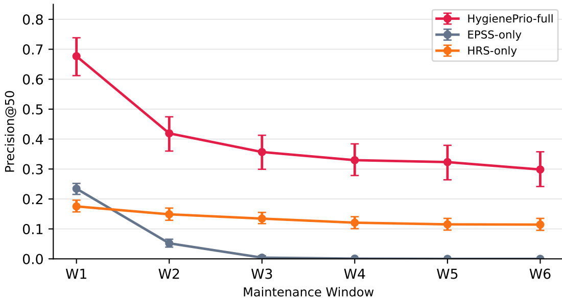
P@50 across 6 bi-weekly windows (25 seeds, synthetic)
