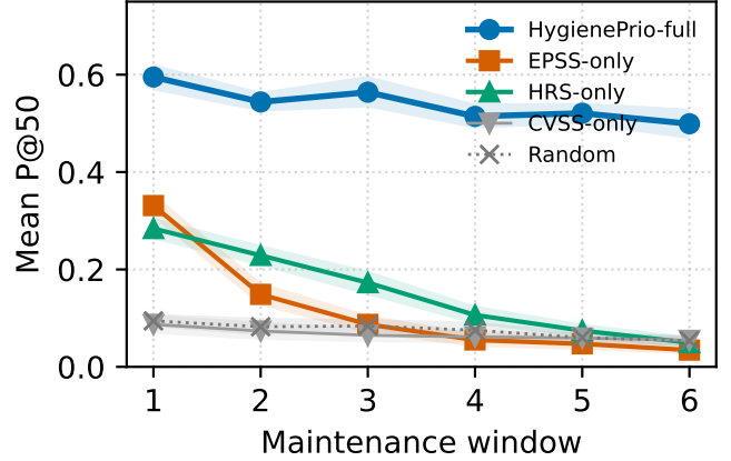
Fig. 1. Mean P@50 per method across six bi-weekly maintenance windows (25 evaluation seeds; shaded bands are 95% bootstrap CIs). HygienePrio-full holds \approx 0.5 throughout; EPSS-only decays 0.331 \rightarrow 0.034; HRS-only crosses above EPSS-only at Window 2.
