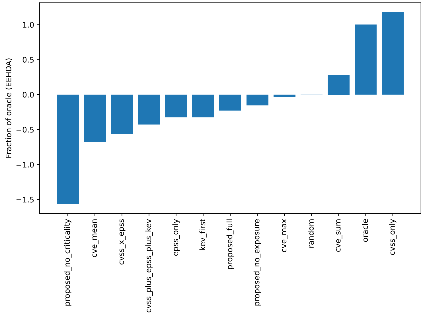
EEHDA fraction-of-oracle by strategy (observed values)
