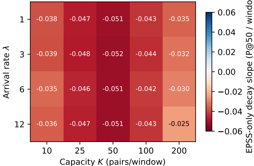
EPSS-only decay slope across ( K, \lambda )
