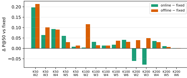
Fig. 2. Per-(K, window) absolute P@50 gain over fixed weights for online (green) and offline (orange) calibration. Negative online bars at K = 200 , w \in \{2, 3\} are the H1 failures.
