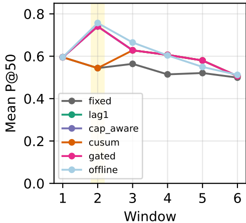
K = 50
