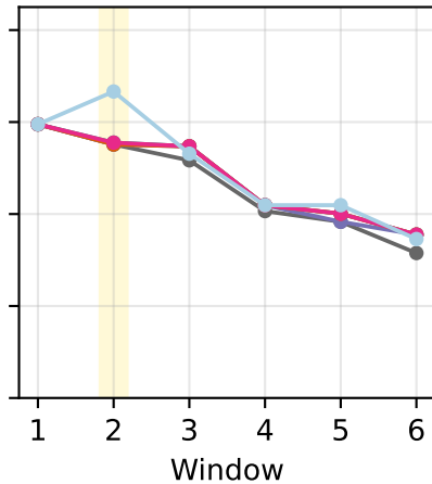
K = 100
