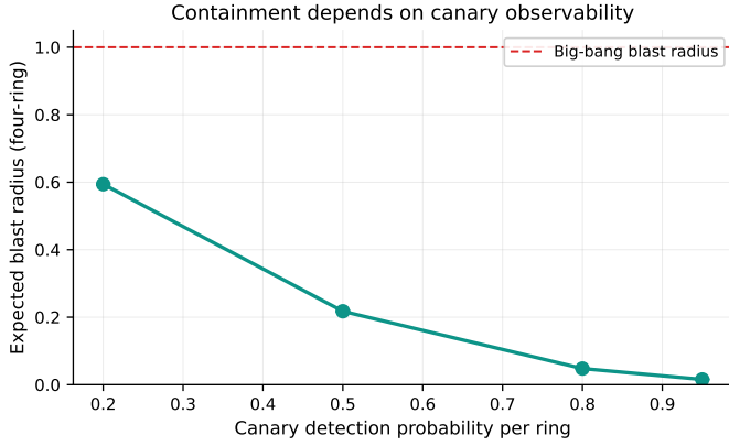
Fig. 2. The four-ring expected blast radius rises from 0.0156 toward the big-bang value as the per-stage detection probability falls from 0.95 to 0.2.
