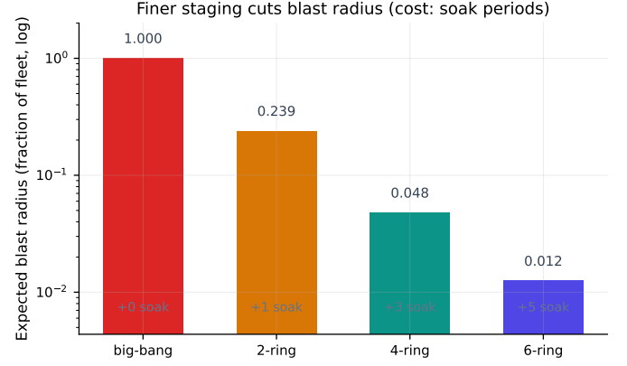
Fig. 1. Expected blast radius (log scale) by rollout granularity at detection probability 0.80; finer staging lowers it from 1.0 at big-bang to 0.0125 at six rings, with marginal reductions of 0.761, 0.1912, and 0.0353 at the labelled convergence cost.
