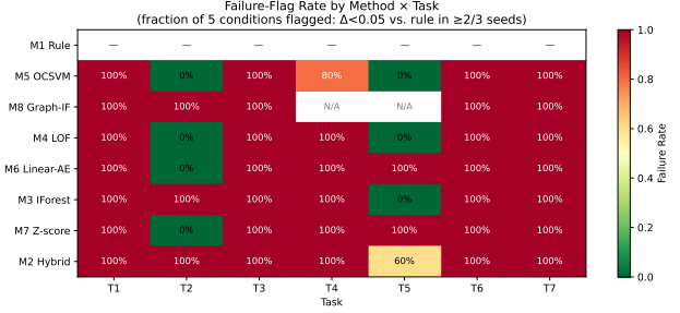
Fig. 1. Failure-flag rate heatmap (method \times task). Red cells indicate flagged configurations, ML fails to improve on the rule baseline by the pre-registered \Delta=0.05 threshold (Eq. (1)) in \geq 2/3 seeds; white cells (M8, T4-T5) are not applicable.
