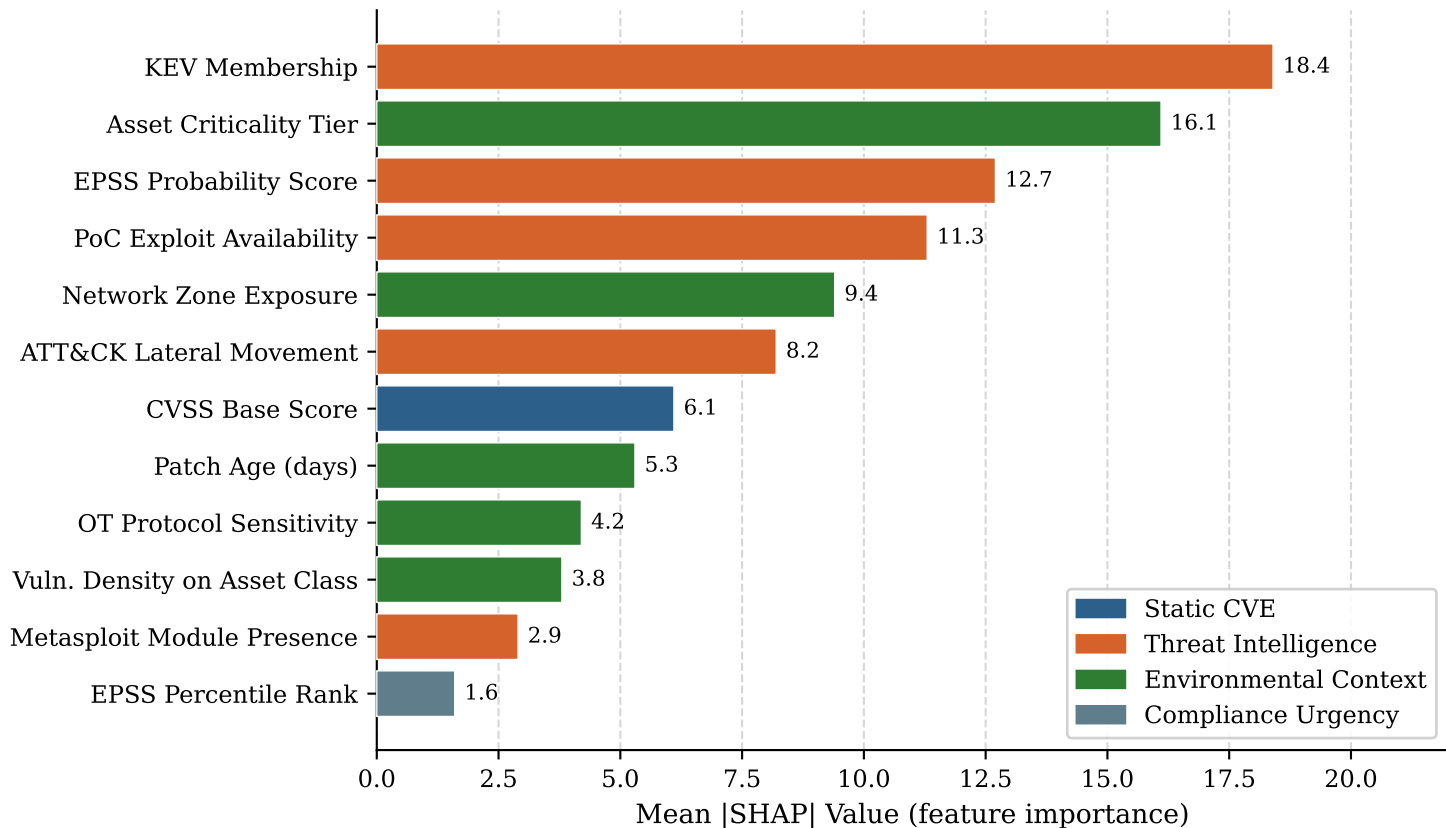
SHAP Global Feature Importance — Top 12 Features
