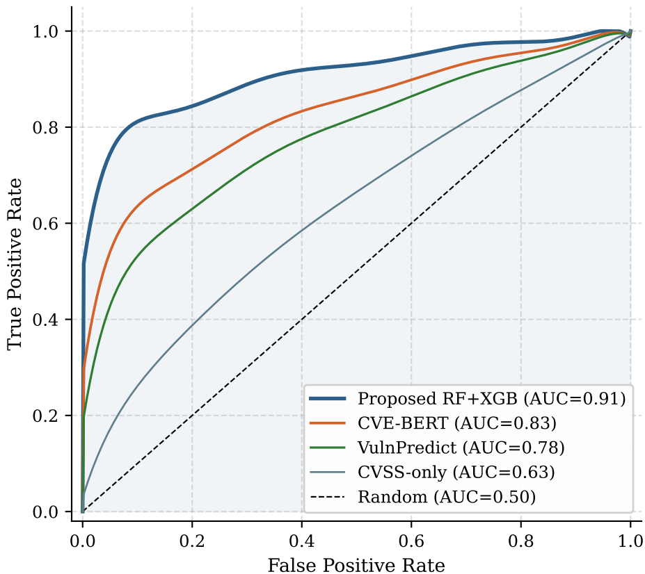
ROC Curves — EPSS Cross-Dataset Validation (12,441 CVEs, Jul-Aug 2024)
