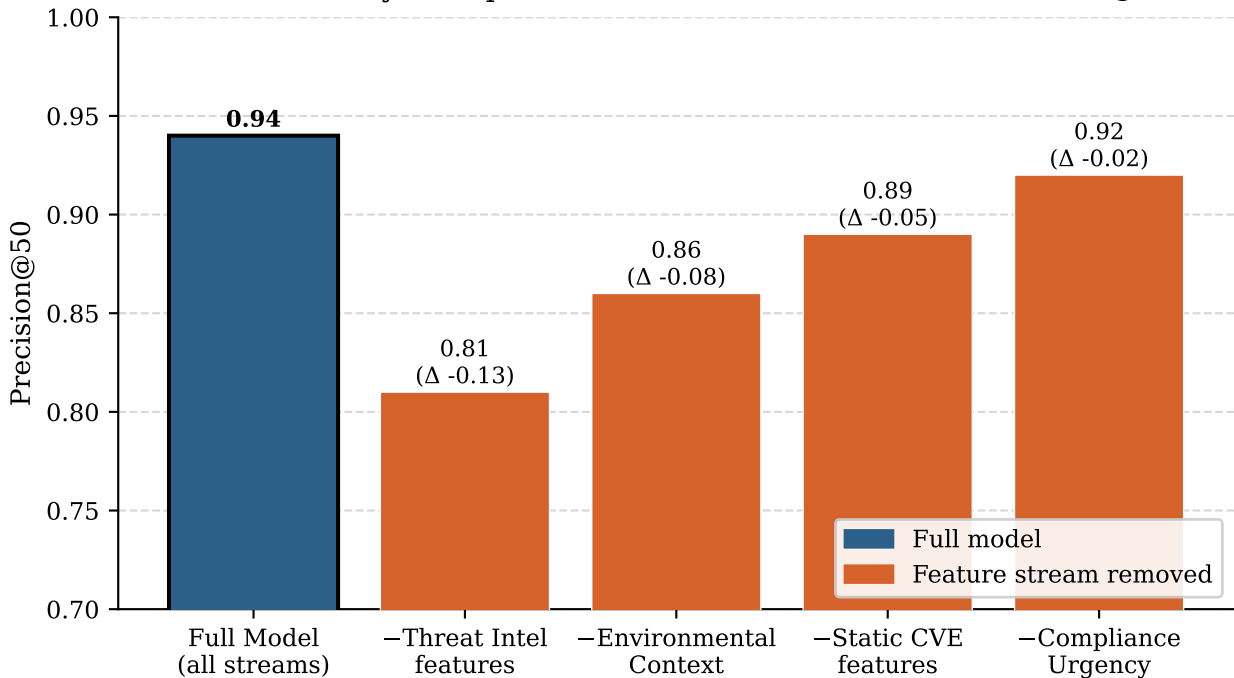
Ablation Study — Impact of Each Feature Stream on Precision@50
