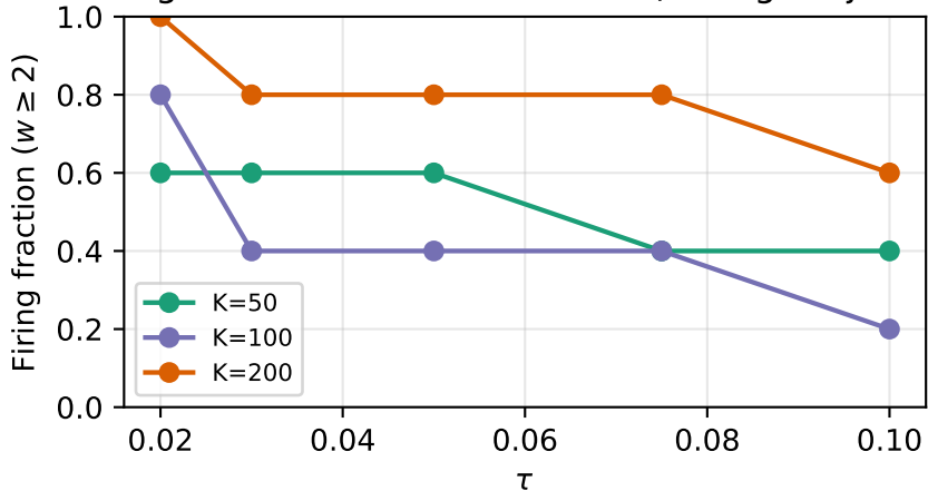
Firing fraction decreases with \tau (H4 sign rejected)
