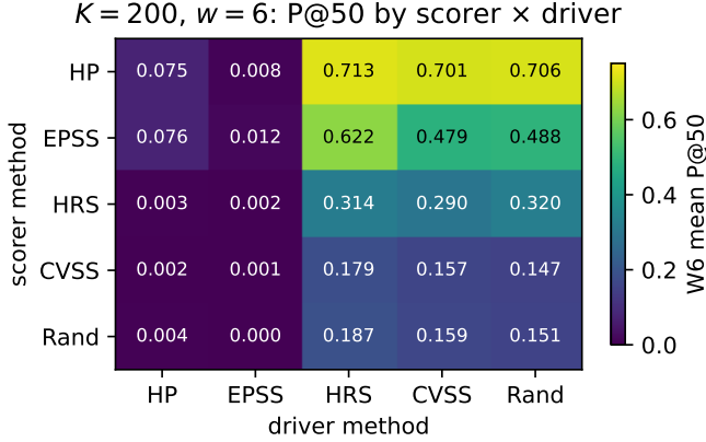
Fig. 2. K = 200 , w = 6 mean P@50 grid. Rows are scoring methods, columns are drivers. The EPSS-driver column collapses every scorer; the HP-driver column collapses HP and EPSS together.
