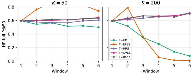
Fig. 1. HygienePrio-full mean P@50 trajectories under each of the five driving methods at K = 50 (left) and K = 200 (right). At K = 200 , the HP-driven trajectory (green) drops to \sim 0.075 by W6 while the three non-draining drivers (CVSS, HRS, Random) hold HygienePrio above 0.70.
