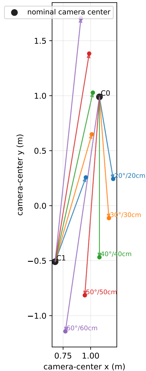
Translation-only camera-center displacement (G2; rotations ignored)
