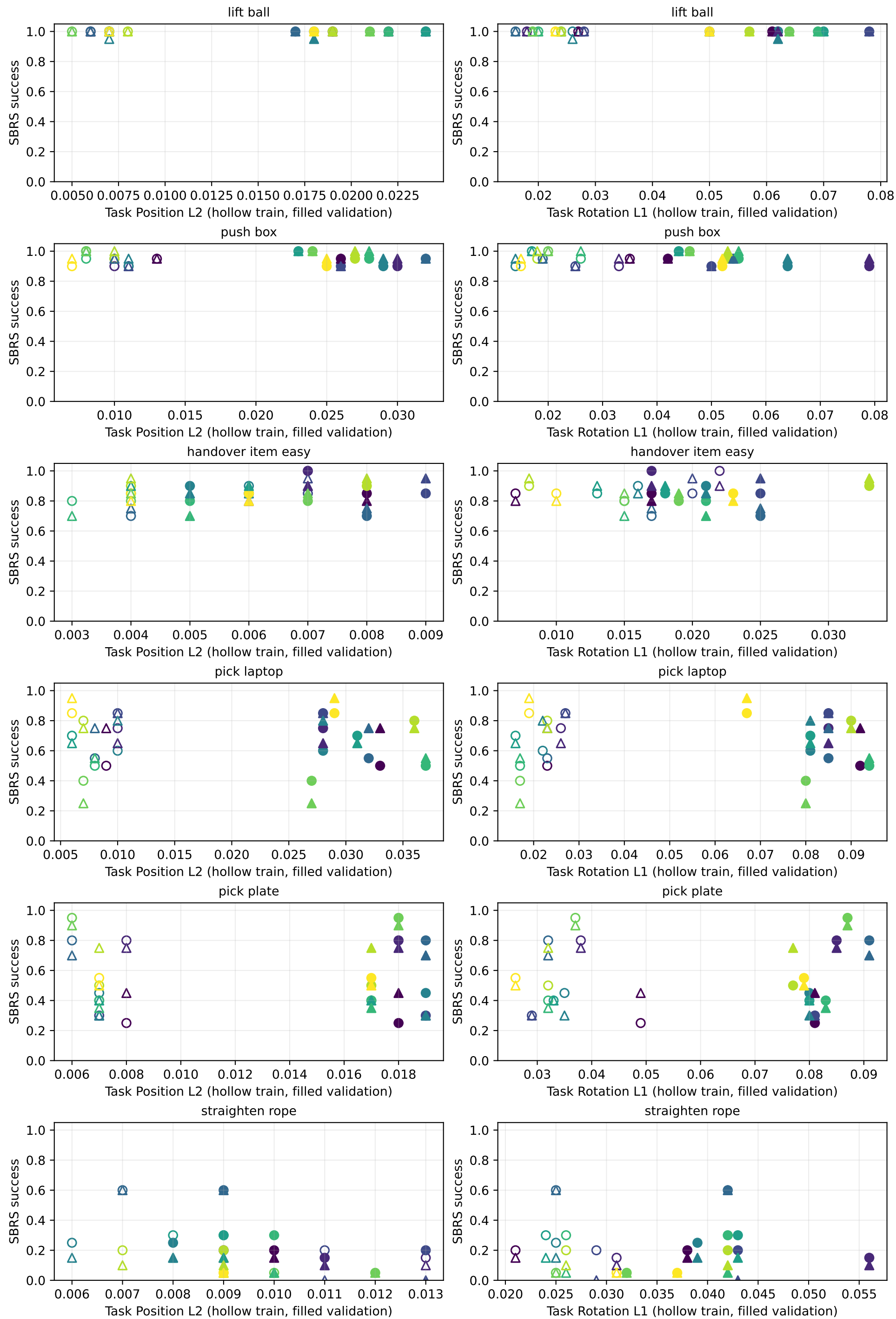
DeltaM task success vs task-level loss ( \circ e0, \triangle e3; hollow train, filled validation; color checkpoint)
