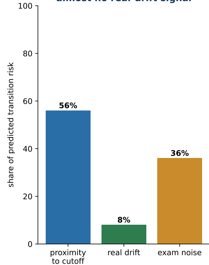
C3 · What transition risk is made of black-box AUROC 0.53: almost no real-drift signal
