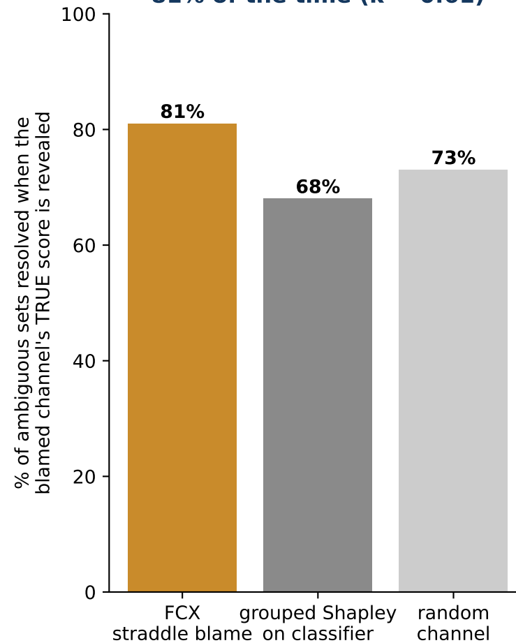
C2 · Why is the set {TD, PIGD}? straddle matches the conformal set 81% of the time ( \kappa = 0.61 )
