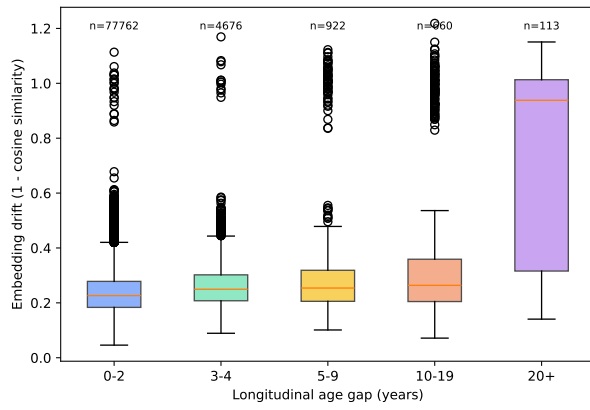
Fig. 4. Pair-level drift by longitudinal age gap group. Drift increased observedly with age gap in the evaluated MORPH sample. The 20+ year group is shown as an extended-tail case with a limited number of pairs.
