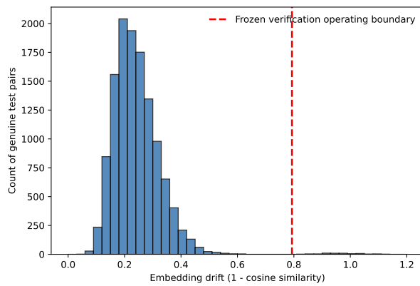
Fig. 6. Observed drift distribution for genuine test pairs and the frozen verification operating boundary at drift = 0.793229669333. This boundary is a verification operating point, not a validated re-enrollment threshold.
