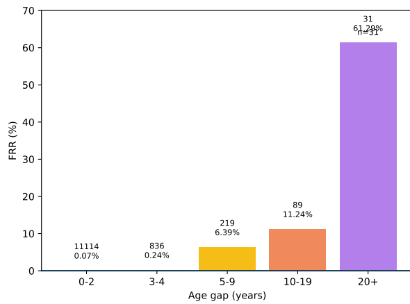
Fig. 5. Test-set FRR across age-gap groups. Larger longitudinal separation was associated with higher genuine verification failure in this evaluated sample. The 20+ year group contains only 31 pairs.
