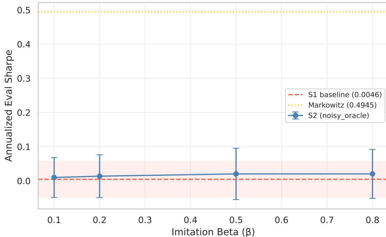
RQ2: S2 vs S1 — predictor=noisy_oracle
