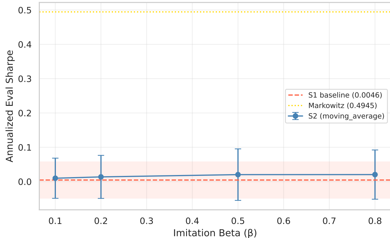
RQ2: S2 vs S1 — predictor=moving_average
