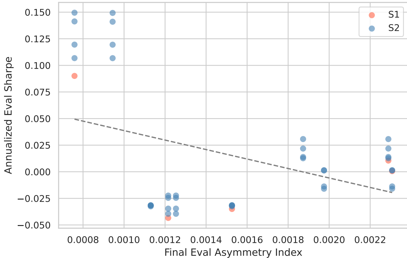
RQ3: Asymmetry vs Sharpe Pearson r=-0.404 ( p=0.006 ), Spearman \rho=-0.119 ( p=0.436 )
