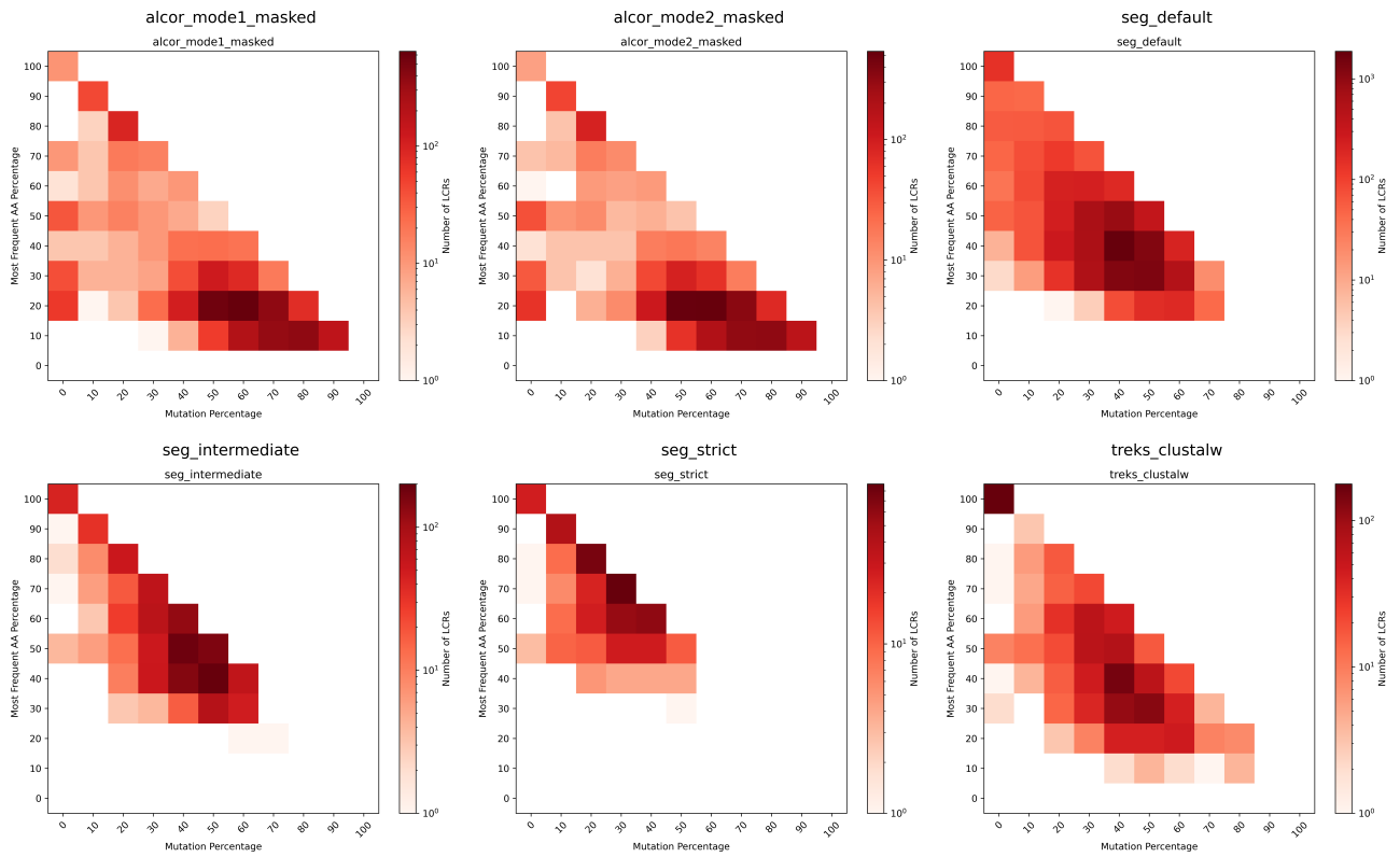
Relationship between amino acid composition and mutation percentage
