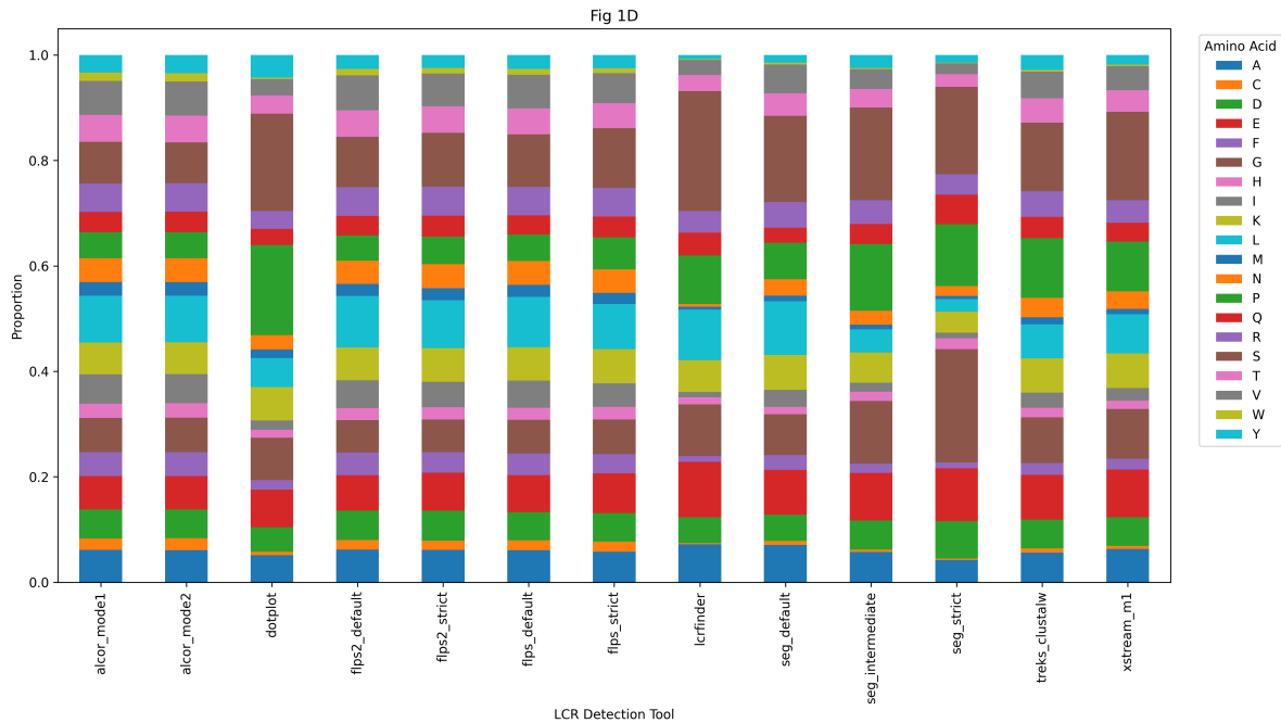
Stacked bar plot of the overall amino acid composition of LCRs detected by each method.
