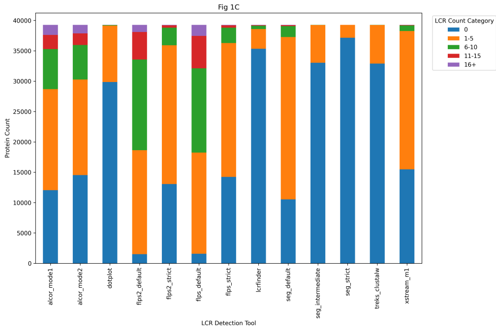
Stacked bar plot comparing the number of LCRs detected per protein by each method, in categories of 0, 1-5, 6-10, 11-15 and above 15.
