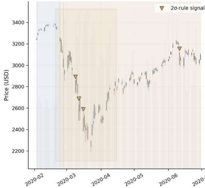
(a) S&P 500 - COVID-19 Crash Overview
