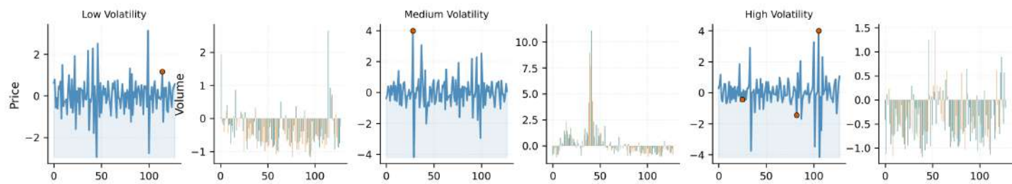
Representative 128-Day Windows Across Volatility Regimes
