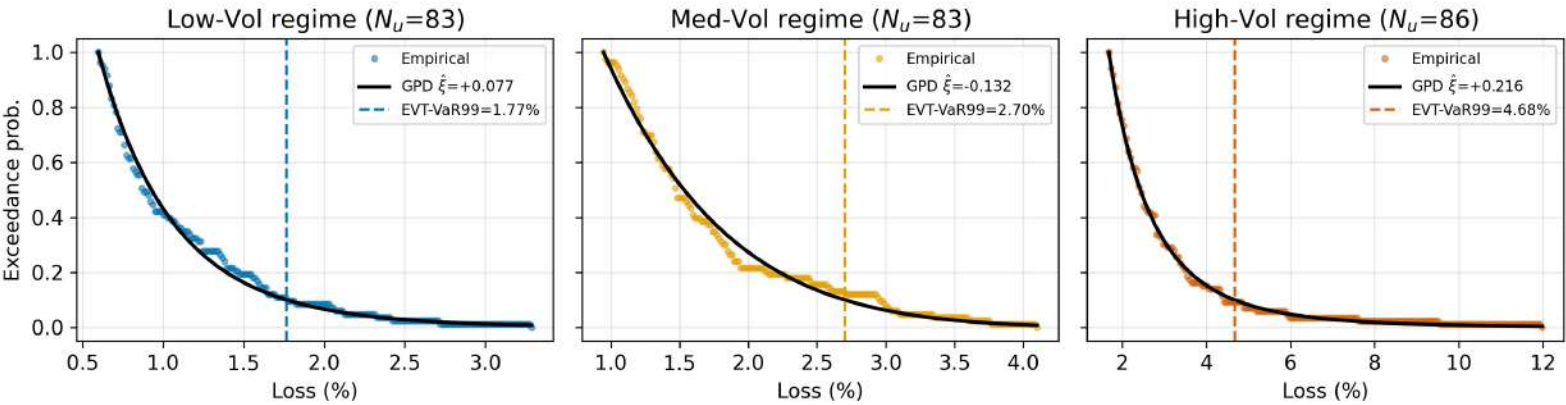
EVT Peak-Over-Threshold Tail Fit by Volatility Regime (S&P 500, 2016--2025)
