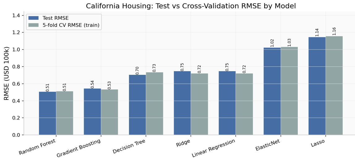
Figure 5. California Housing: test vs CV RMSE. Ensembles dominate; Lasso/Elastic Net collapse to the mean baseline at \alpha = 0.001 .
