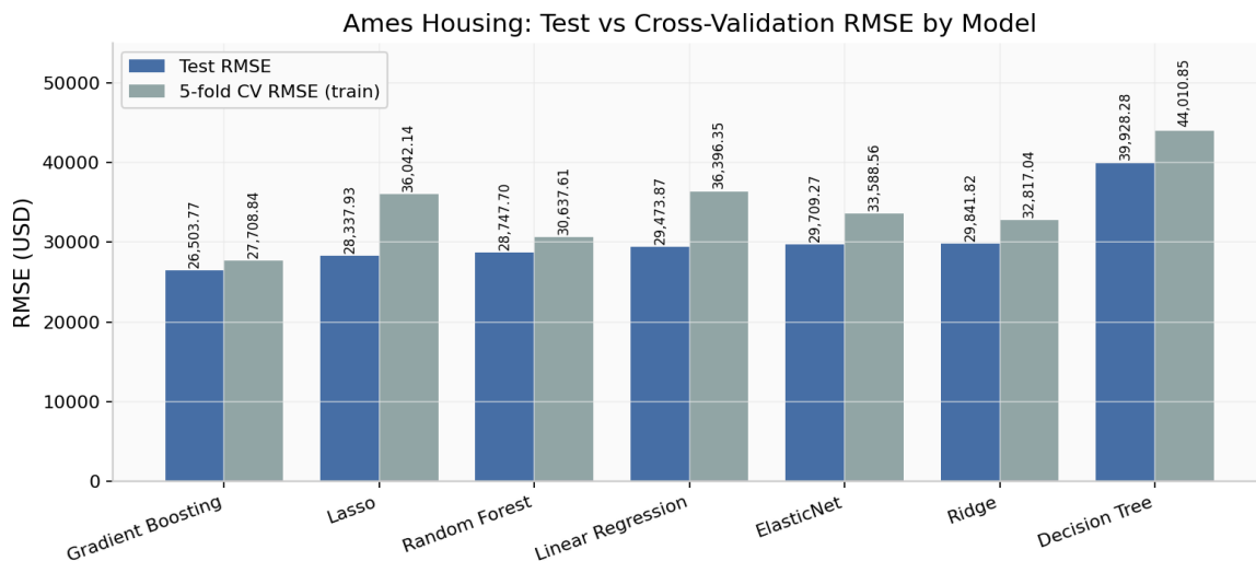
Figure 4. Ames Housing: test vs 5-fold CV RMSE. Gradient Boosting leads on both; the CV–test gap is small, indicating stable selection.
