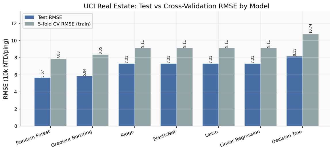
Figure 6. UCI Real Estate: test vs CV RMSE. The linear family is nearly identical across all four variants on this small dataset.
