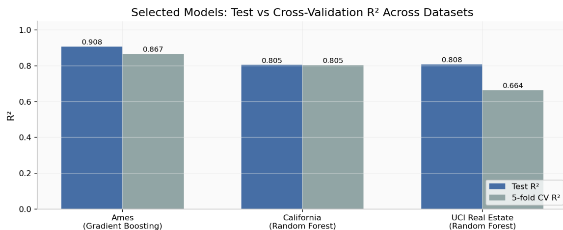
Figure 7. Selected models: test vs cross-validation R^2 across the three datasets.
