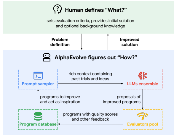
Figure 1 | AlphaEvolve high-level overview.
