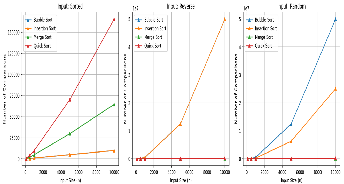
Number of Comparisons vs Input Size
