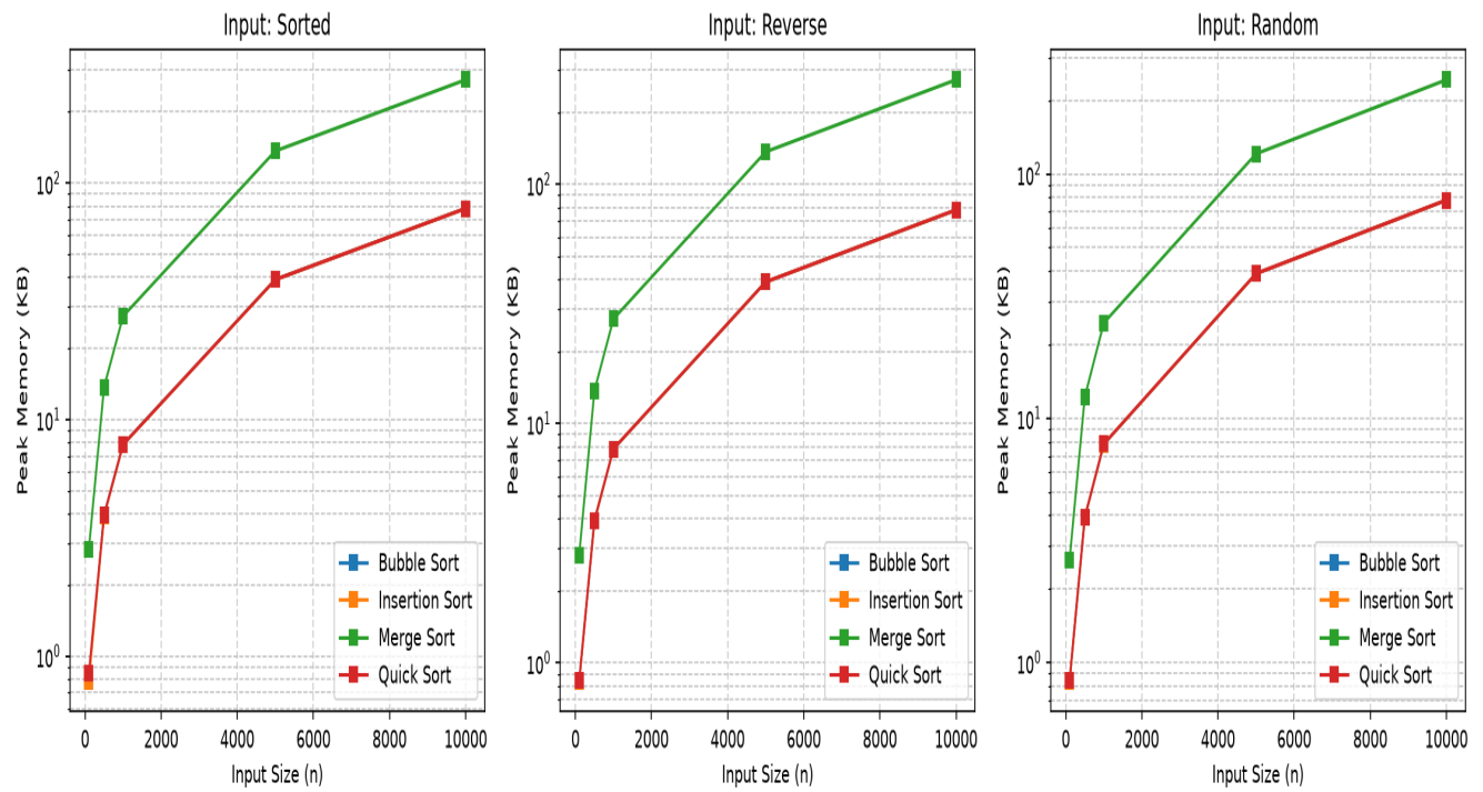
Sorting Algorithm Memory Usage vs Input Size (Log Scale)
