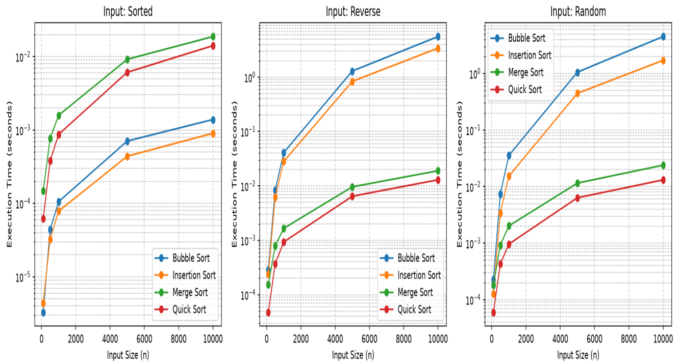
Sorting Algorithm Execution Time vs Input Size (Log Scale)
